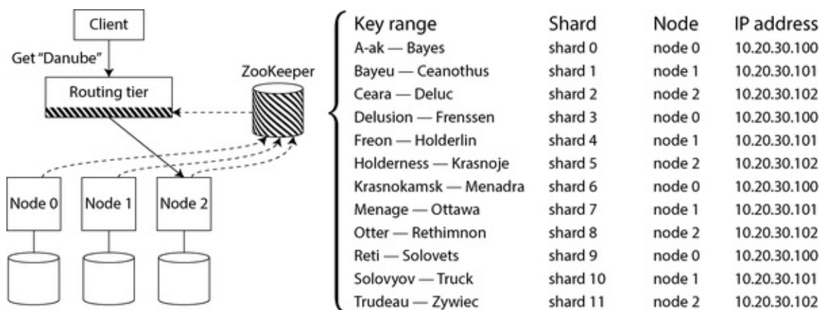
Figure 7-8. Using ZooKeeper to keep track of the assignment of shards to nodes
