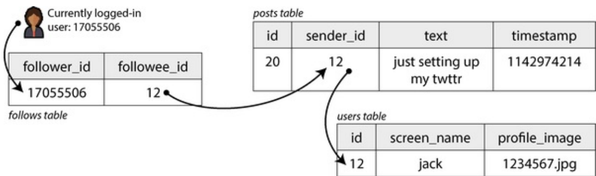
Figure 2-1. A simple relational schema for a social network in which users can follow one another
