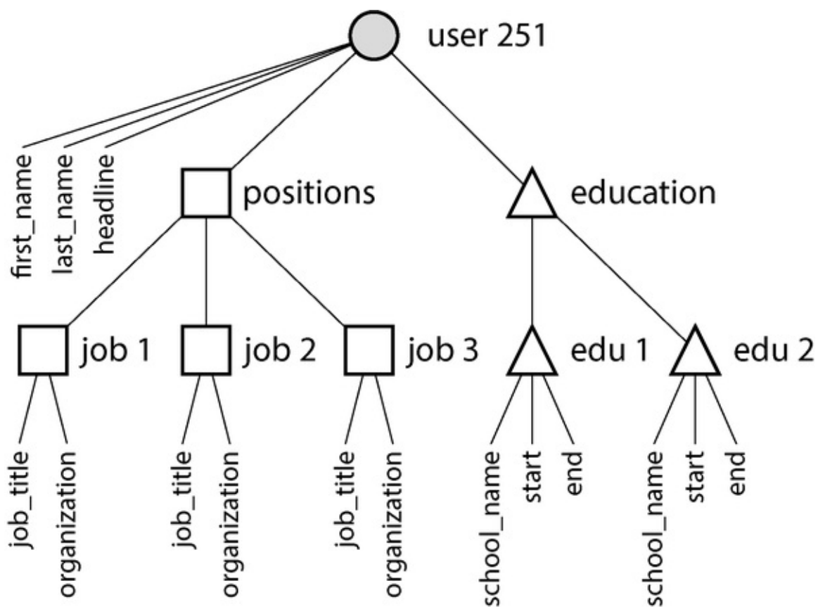
Figure 3-2. One-to-many relationships forming a tree structure
