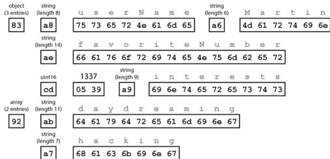
Figure 5-2. Our record (Example 5-2) encoded using MessagePack
