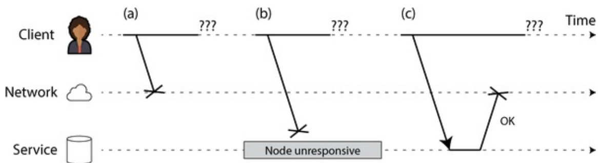
Figure 9-1. If you send a request and don't get a response, it's not possible to distinguish whether (a) the
