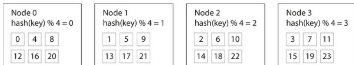
Figure 7-3. Assigning keys to nodes by hashing the key and taking it modulo the number of nodes. Changing
