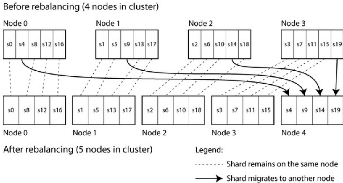
Figure 7-4. Adding a new node to a database cluster with multiple shards per node
